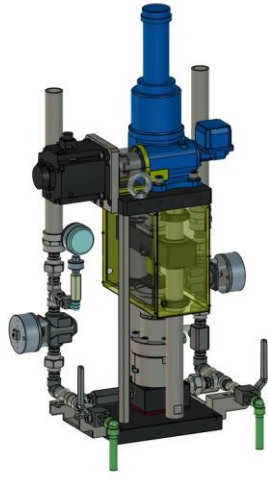
MEASURING CYLINDER ASSY 514cc/shot
